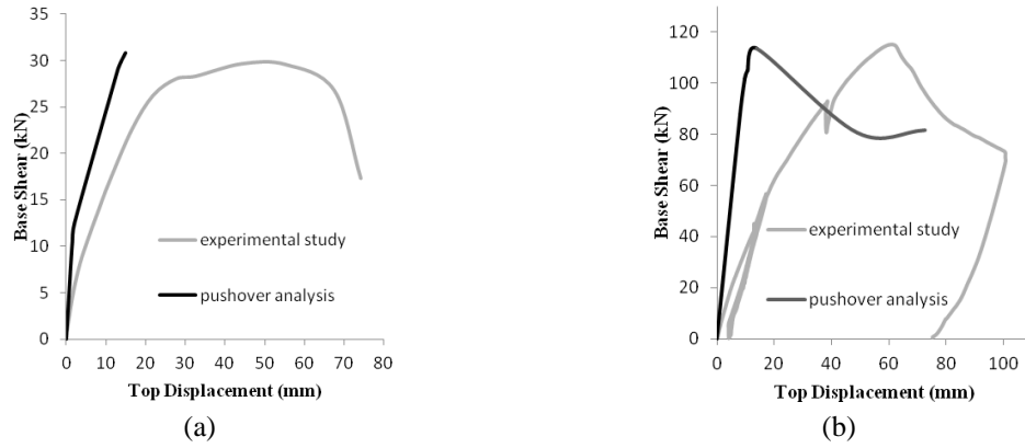
Fig. 9 Lateral load-carrying capacities of analytical and experimental studies: (a) RC frame; (b) 1/2CSBF (-) -X
